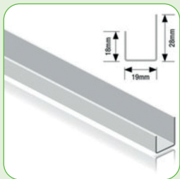
Wall Liner Track
