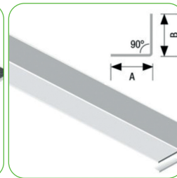
SFS Angles
