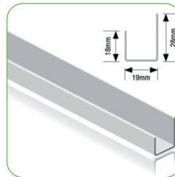
MF6 Perimeter
